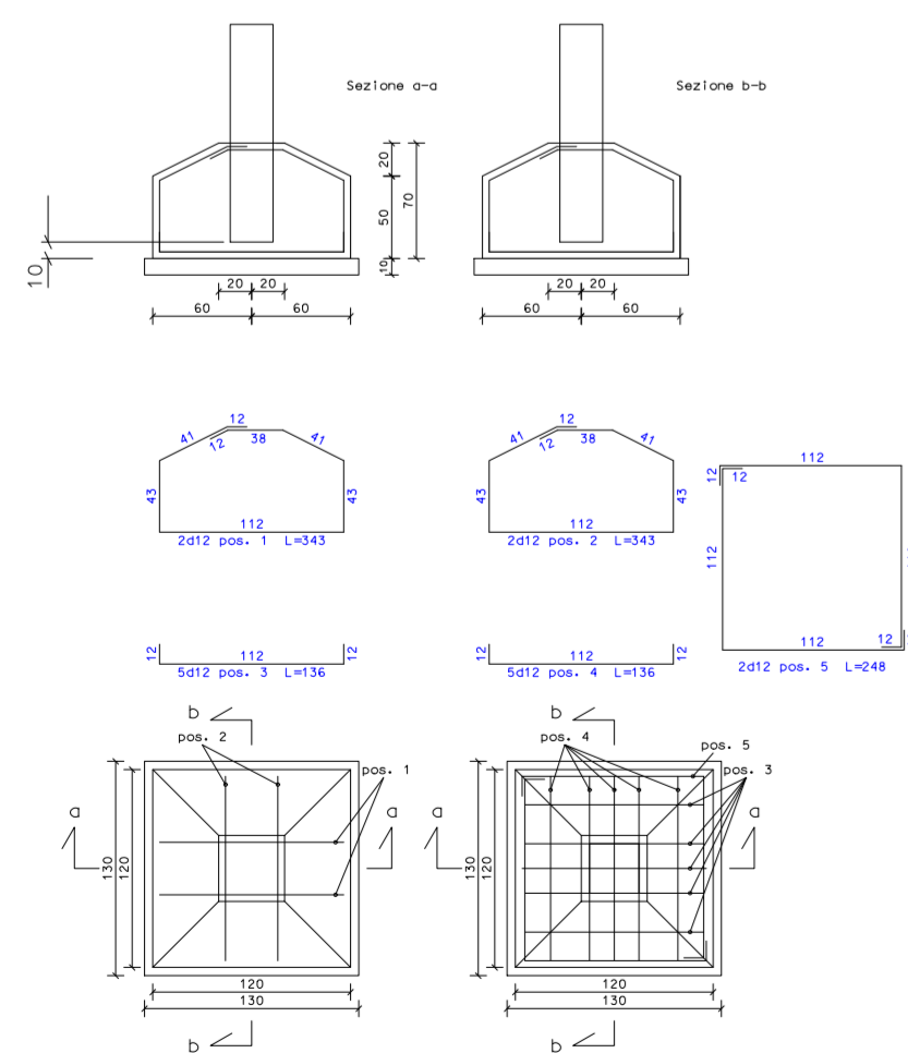
pilotti 2, 3, 17, 18, 32, 33, 47, 48, 62, 63, 77, 78, 92, 93, 107, 108
