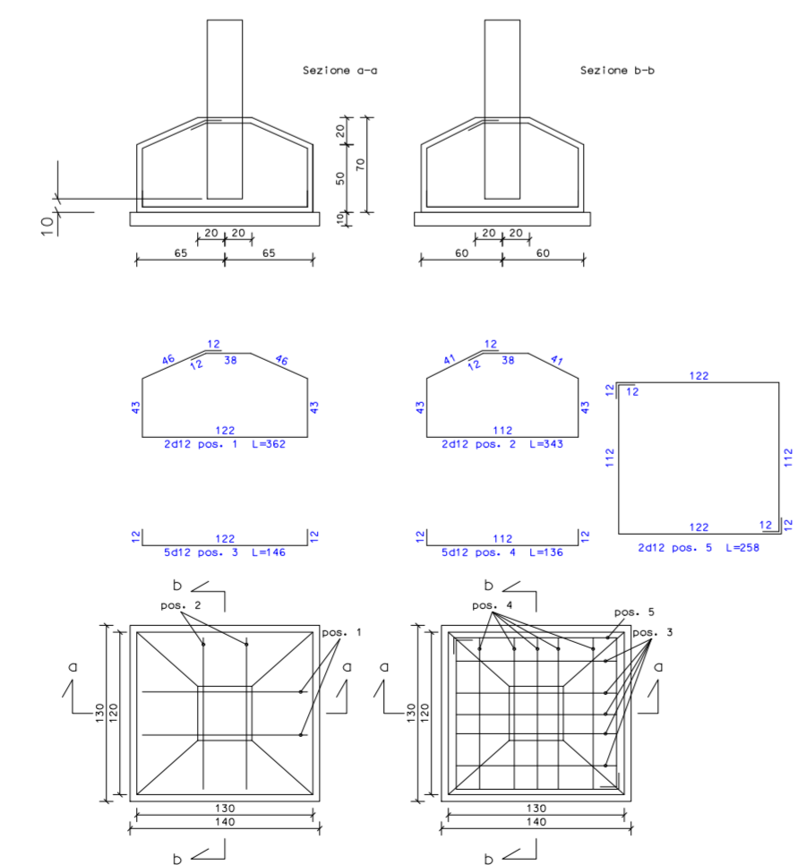
pilotti 1, 4, 16, 19, 31, 34, 46, 49, 61, 64, 76, 79, 91, 94, 106, 109
